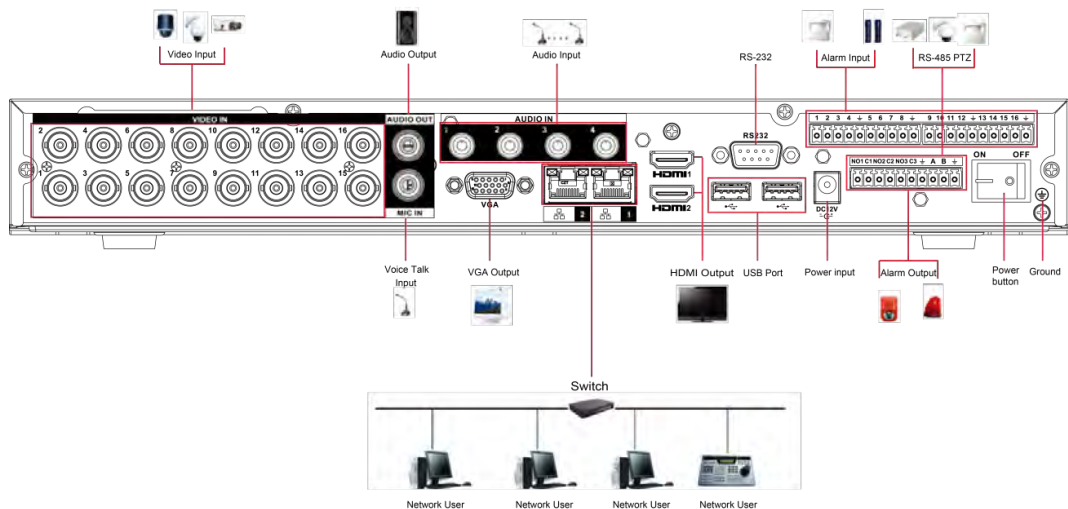
Figure 4-1 Connection diagram
