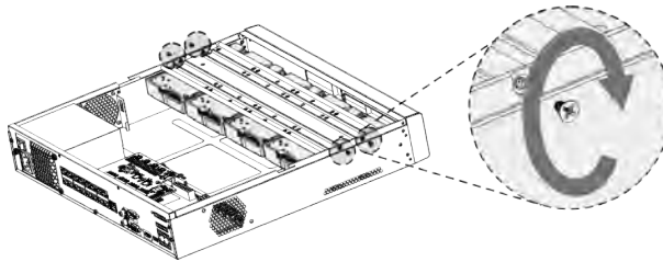
Figure 2-21 Fasten screws
