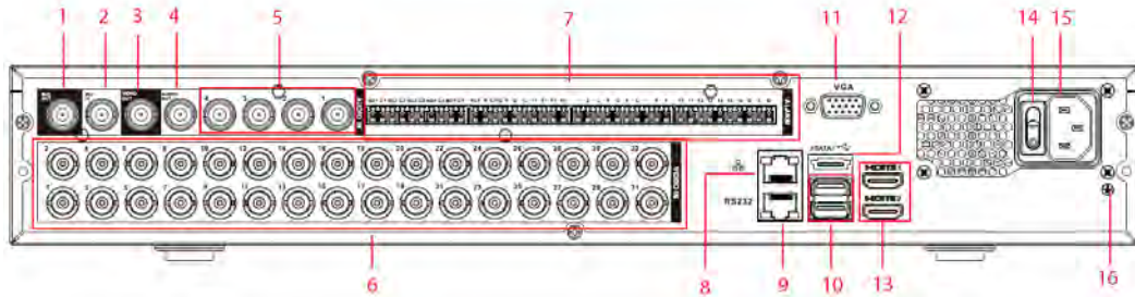
Figure 3-20 Rear panel (2)
