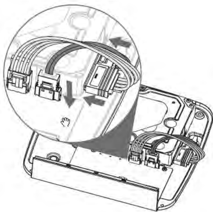
Figure 2-33 Connect cables
