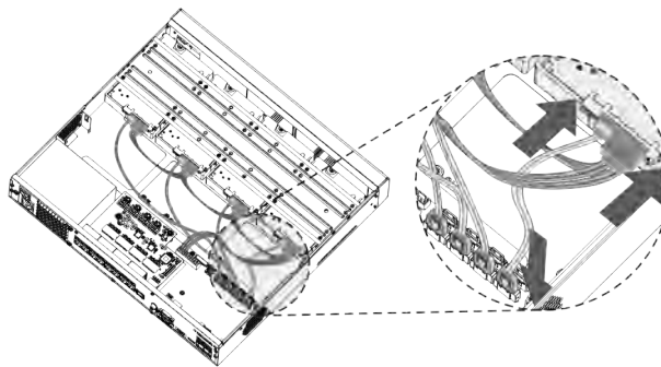
Figure 2-22 Connect cables
