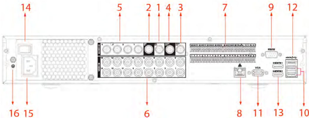
Figure 3-21 Rear panel (3)
